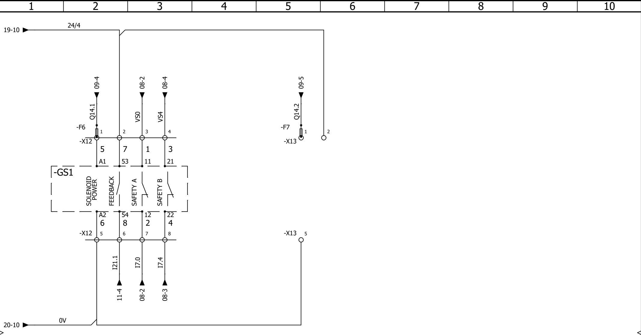
STAGE LEFT DOCK DOOR SAFETY INTERLOCK
